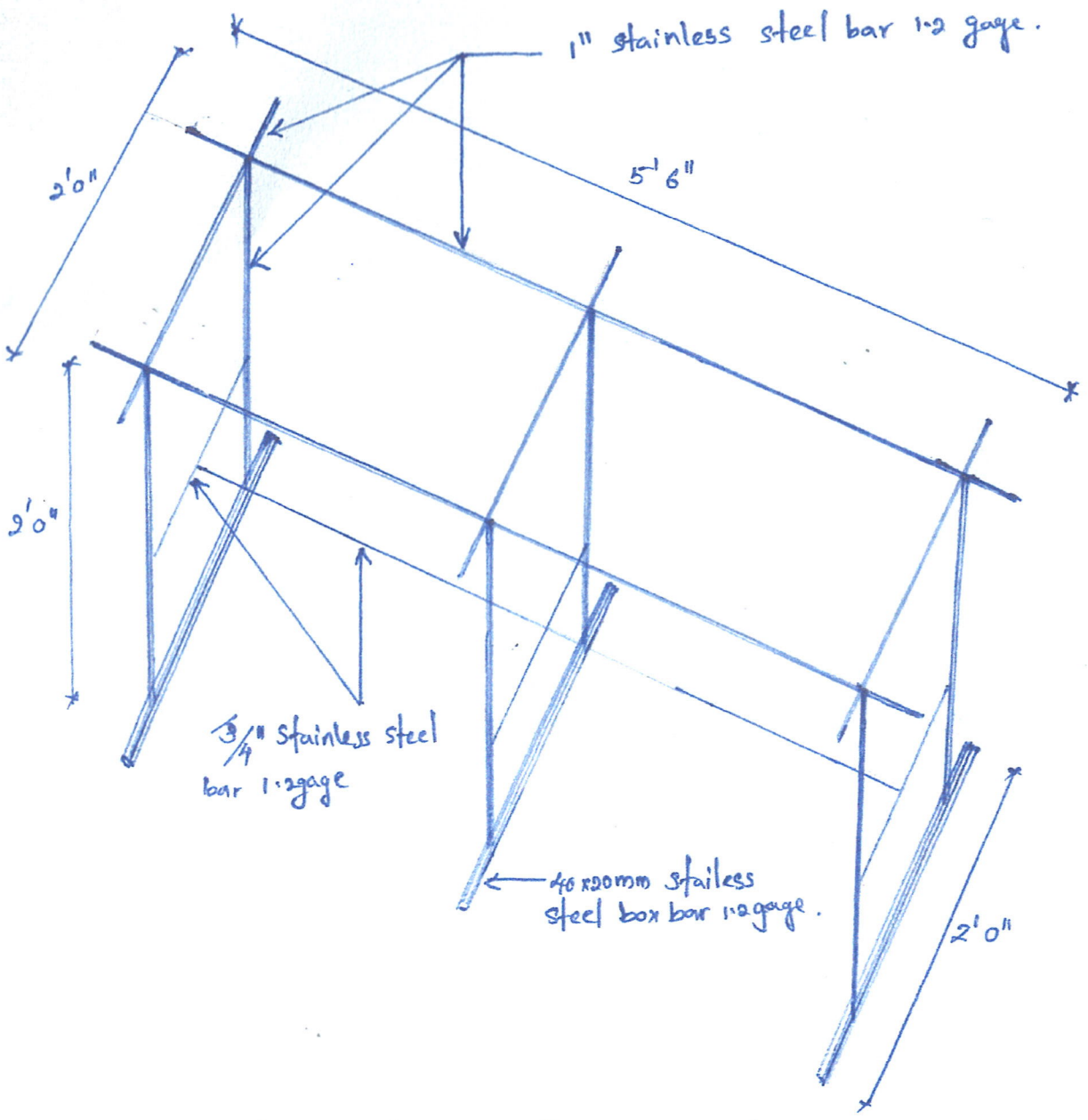
Stainless steel stand for crematorium.
